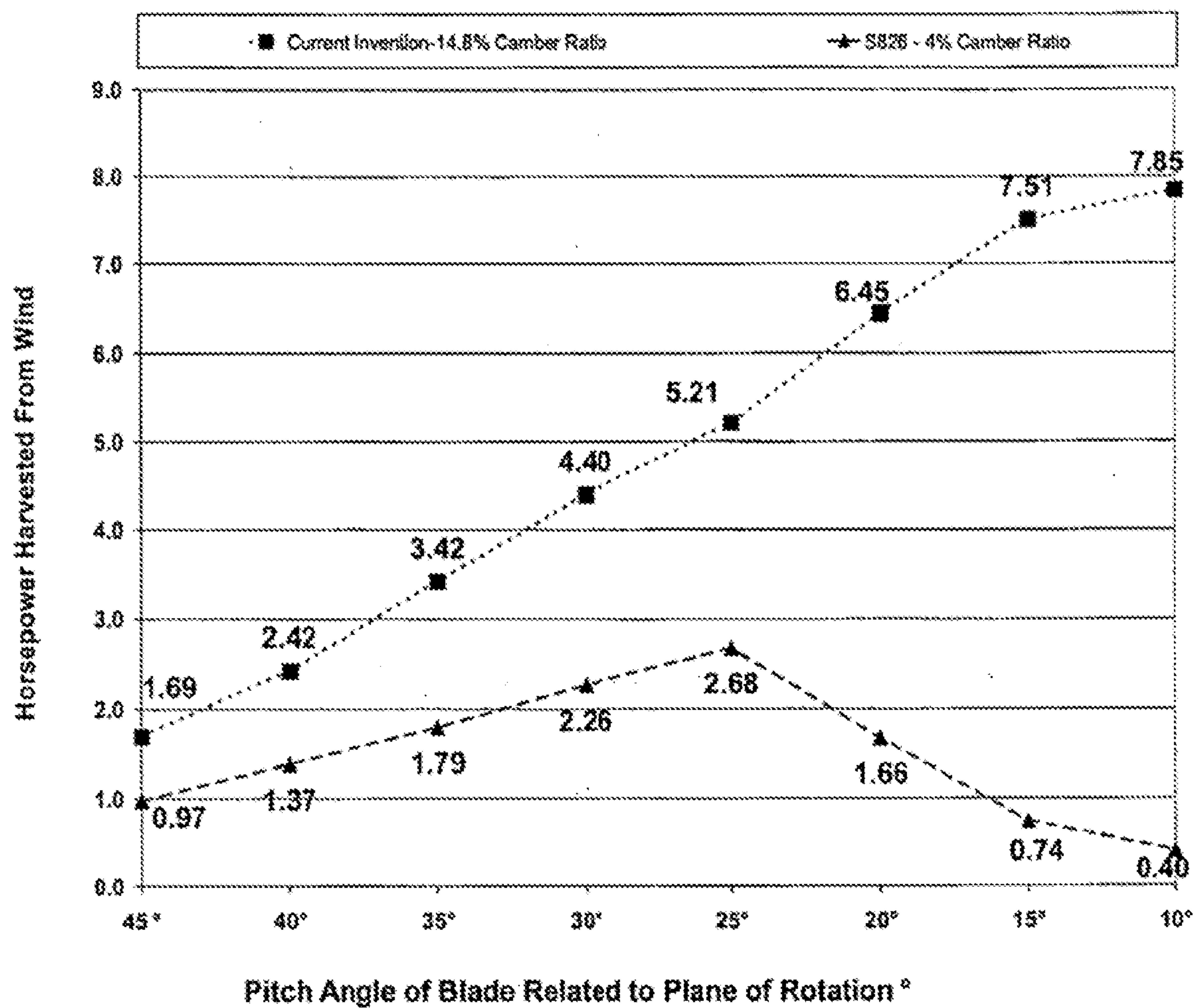
Fig. 4 - Dynamic Wind Tunnel Tests with a Rotating Turbine
