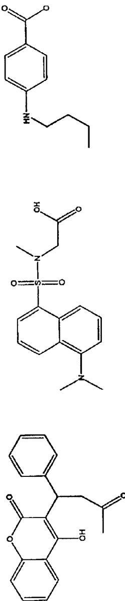
n-butyl-p-aminobenzoate - Site I
