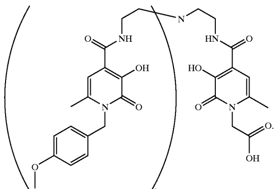
TREN-6-Me-HOPOMOB-HOPOAC
