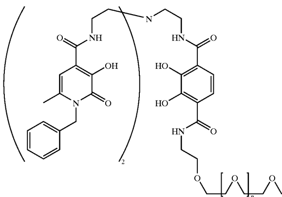
TREN-6-Me-HOPOBn-TAMPEG
