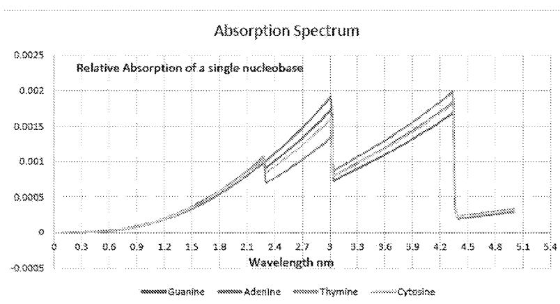
Figure 1. EUV Absorption Spectra of 4 DNA Nucleobases CGAT at normal incidence.
