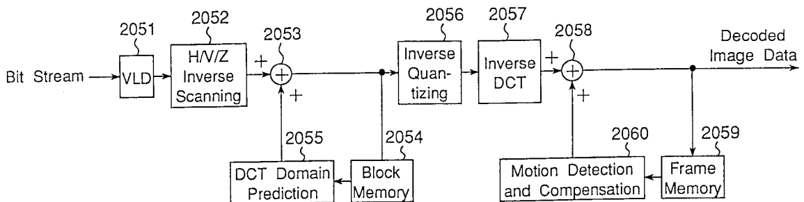
Eighth Preferred Embodiment Image Predictive Decoding Apparatus
