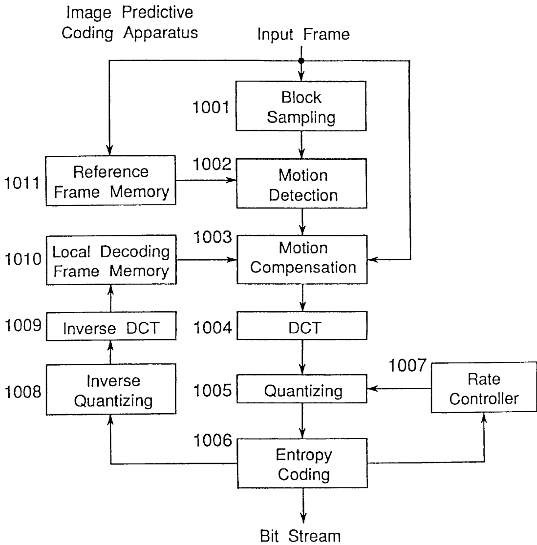
Fig.14 PRIOR ART
