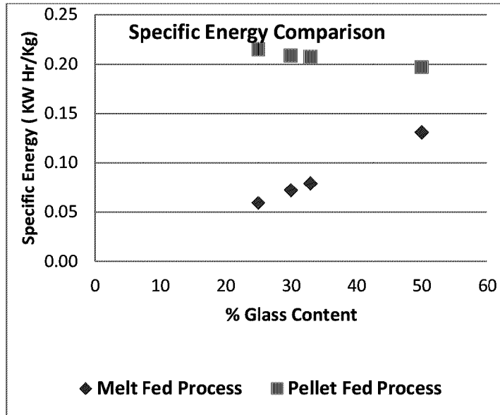
Figure 4. Specific Energy Comparison
