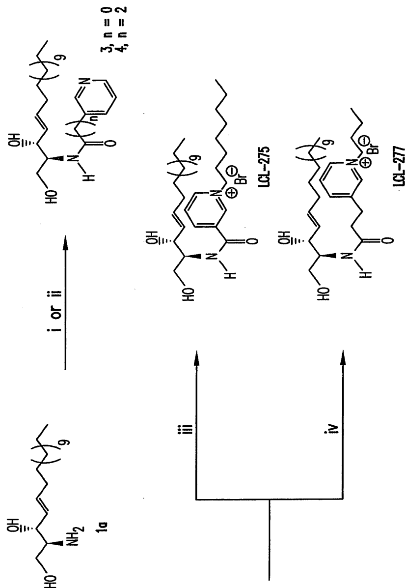
Scheme 2. Synthesis of Class B of Ceramidoids
