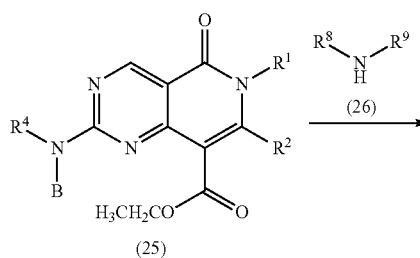
Scheme 8
