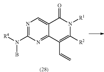
Scheme 9
