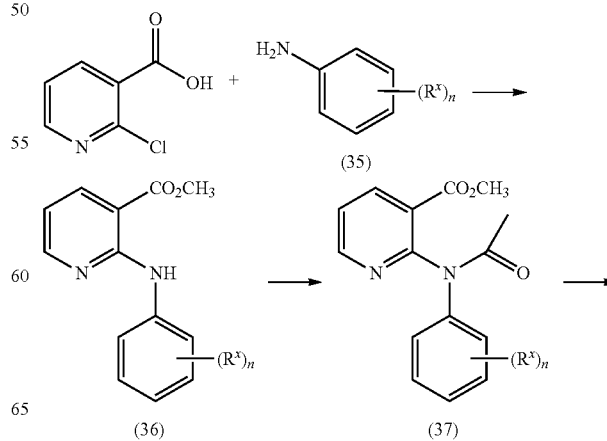
Scheme 12
