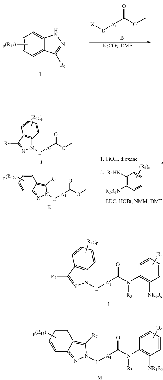
Scheme 2
