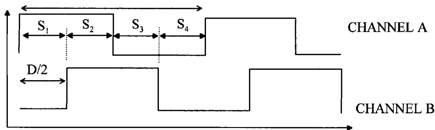
FIGURE 5 (PRIOR ART)
