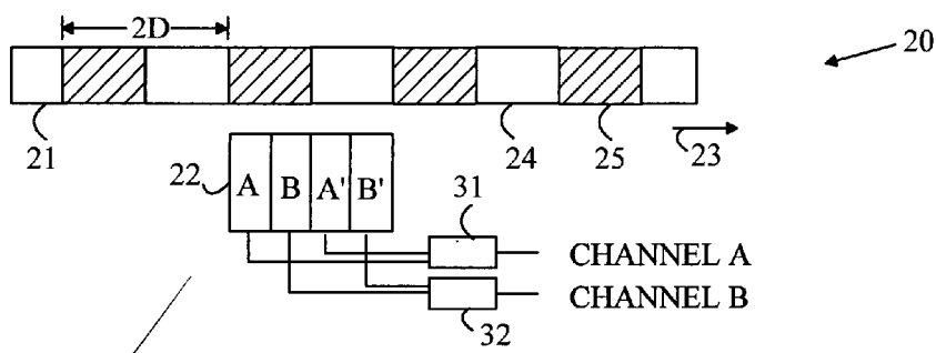
FIGURE 3 (PRIOR ART)
