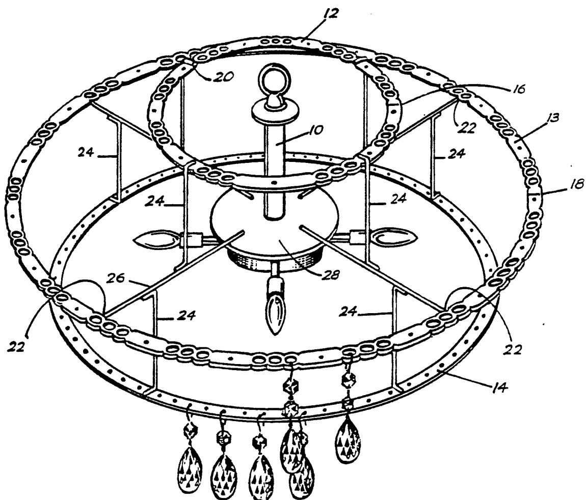
FIG. 1 ( PRIOR ART )
