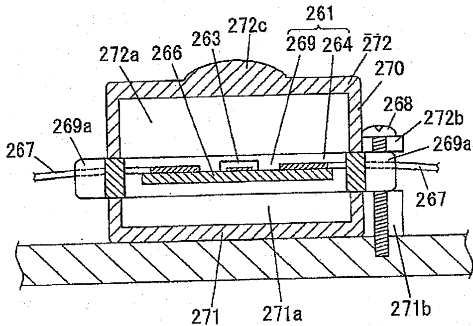
FIG. 19 (PRIOR ART)
