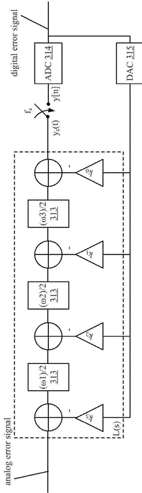
Cascade of Integrators with Distributed Summation (CIFB)
