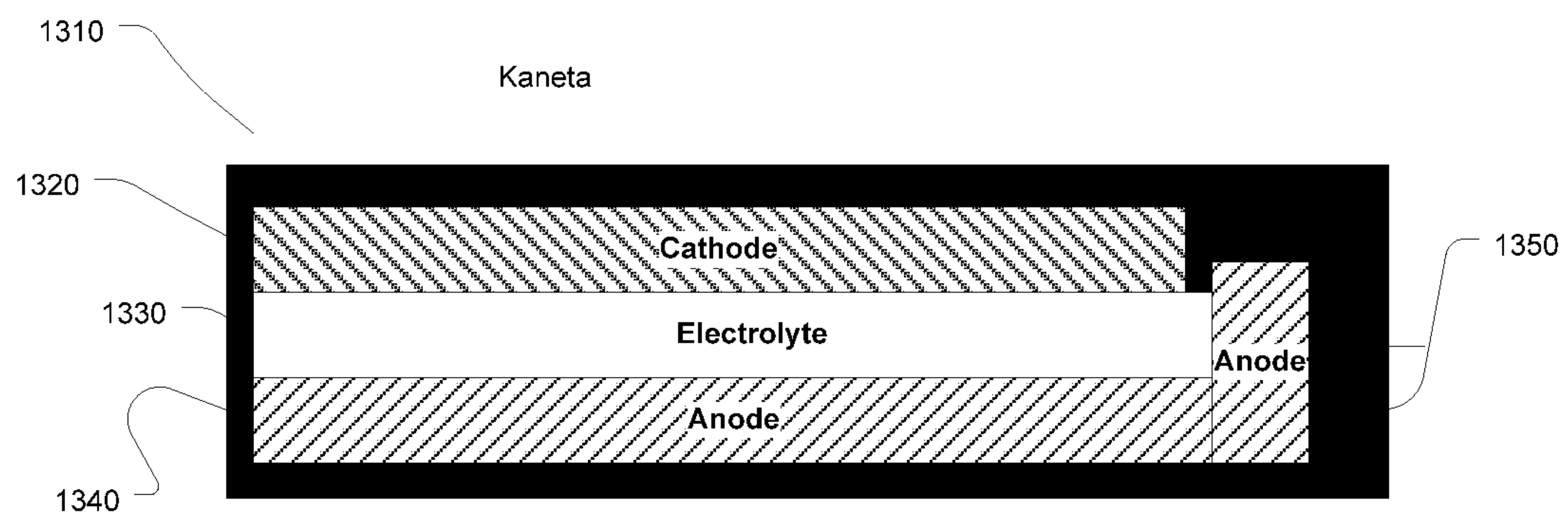
Fig. 13 (Prior Art)
