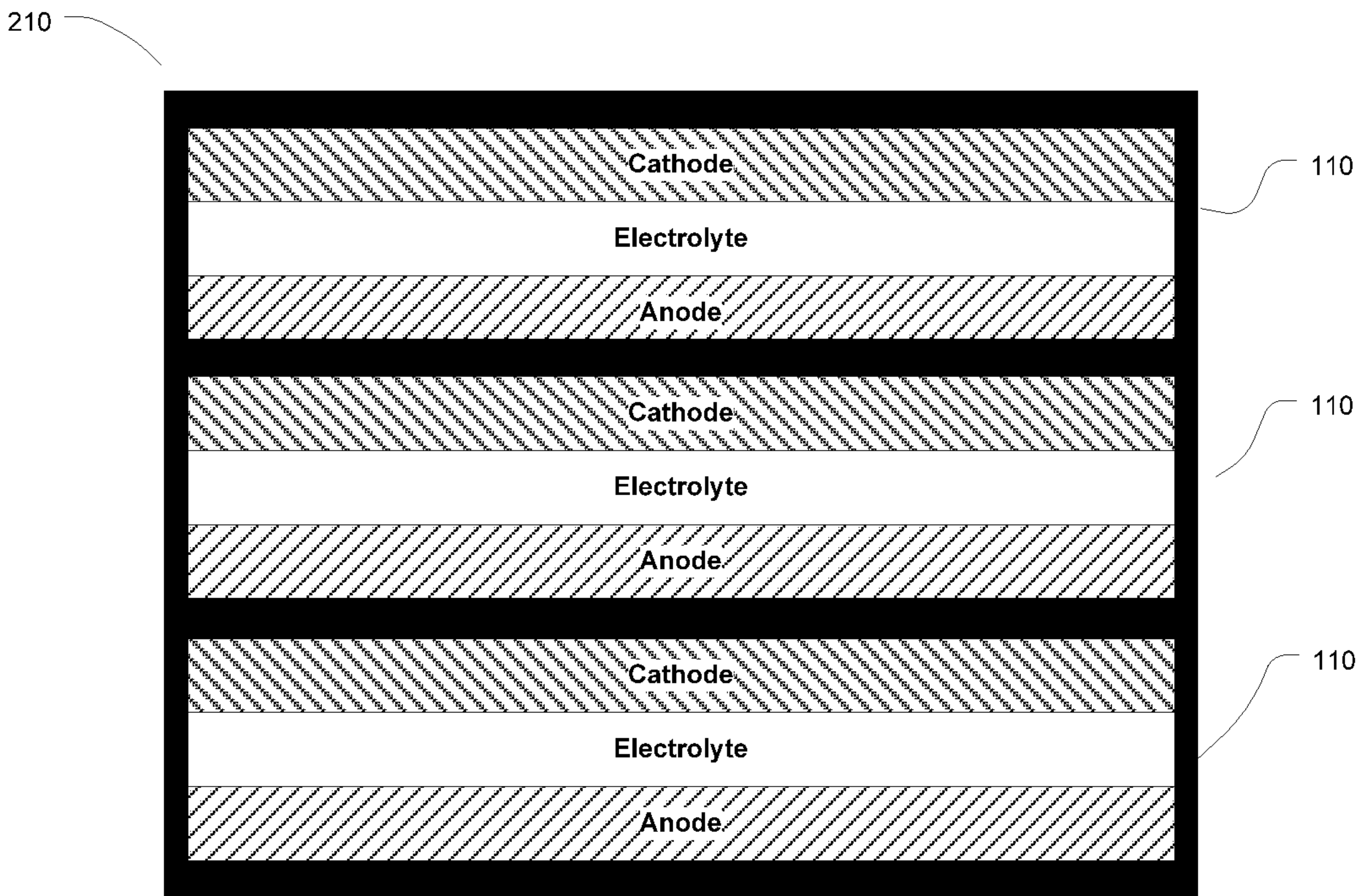
Fig. 2 (Prior Art)
