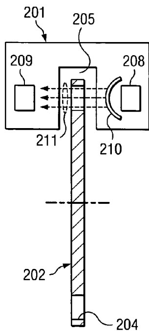
FIG. 2A (PRIOR ART)
