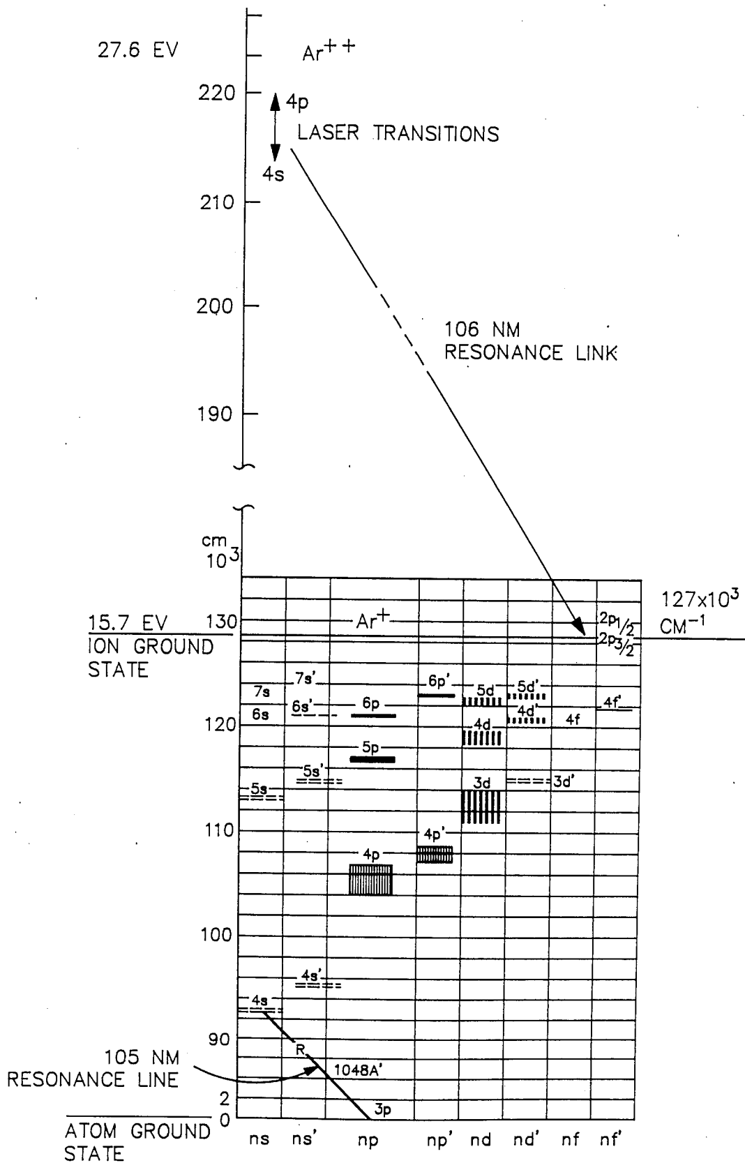
ARGON ION LASER ENERGY LEVELS FIG.1 .
