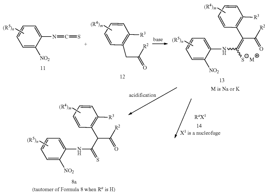
Scheme 6
