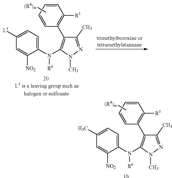
Scheme 11
