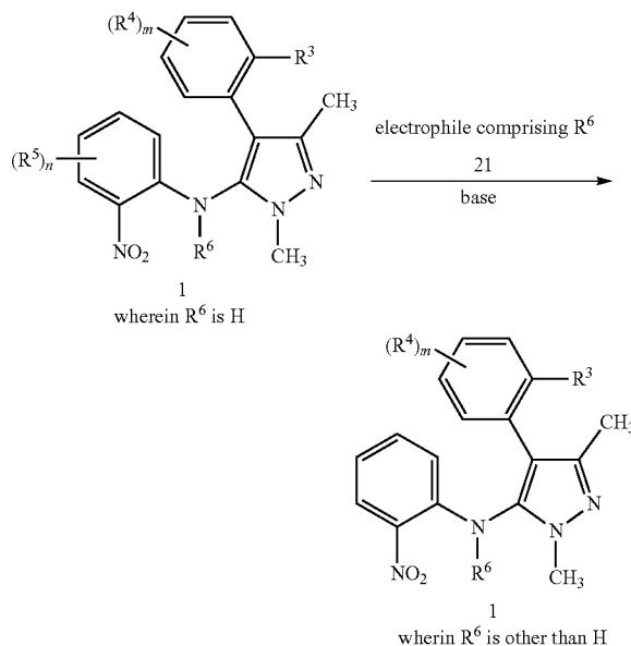
Scheme 12
