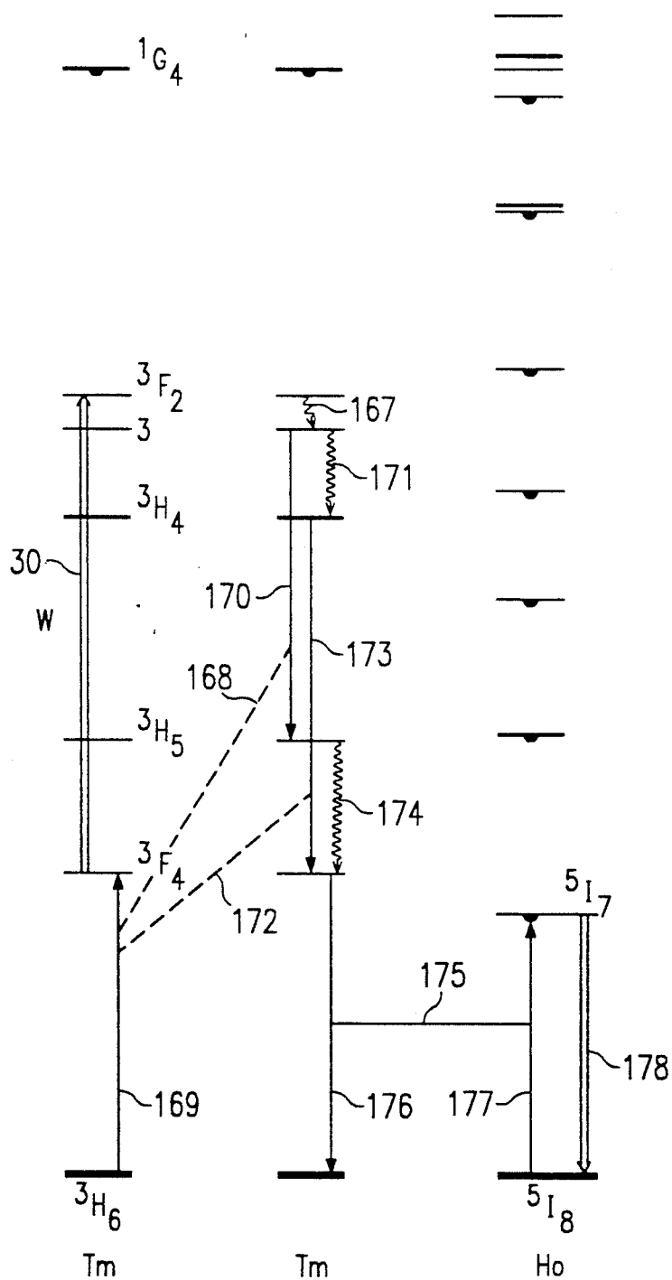
FIG. 12 AVALANCHE DRIVEN THULIUM-HOLMIUM CROSS-PUMPED LASER
