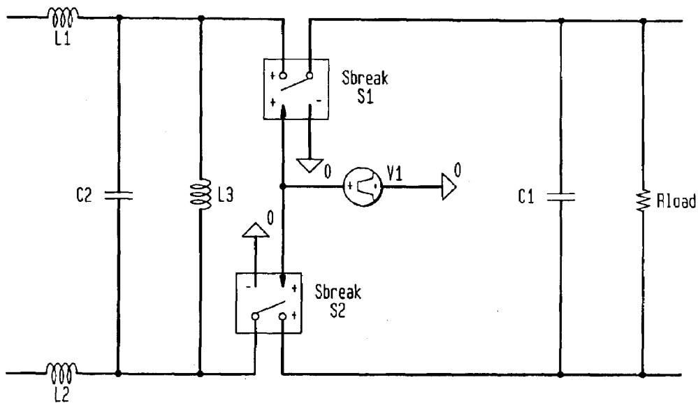
FIG. 242 DIFFERENTIAL CONFIGURATION
