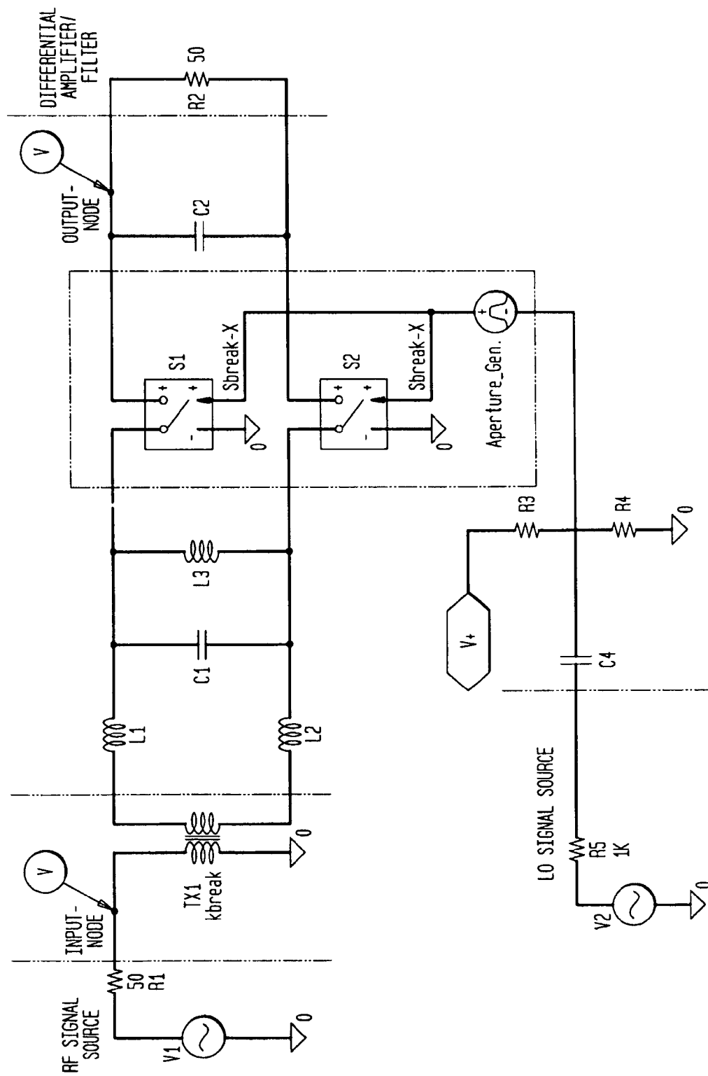
FIG. 261 FULL DIFFERENTIAL
