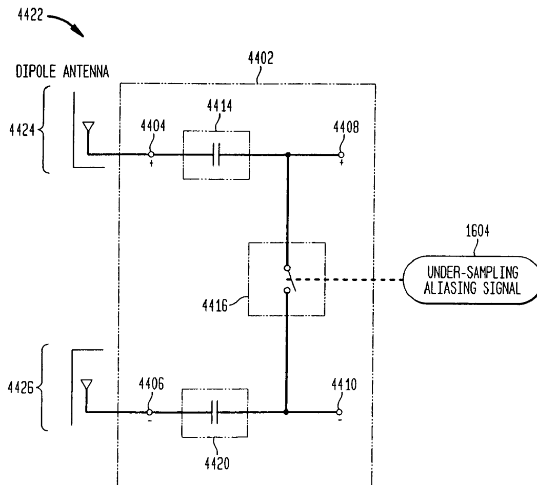
FIG. 44B DIFFERENTIAL INPUT TO DIFFERENTIAL OUTPUT
