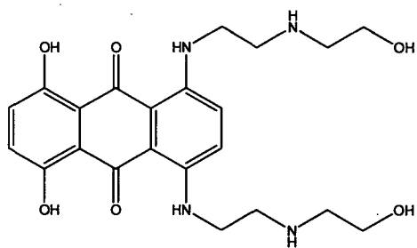
Mitoxantrone
