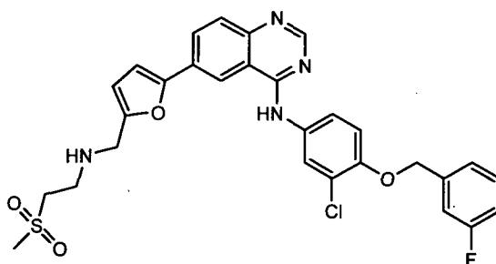
Lapatinib
