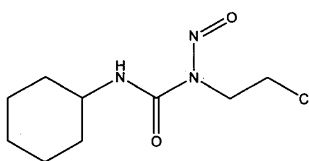
Lomustine
