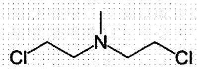
Mechlorethamine
