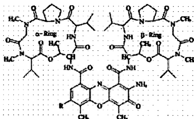
Actinomycin
