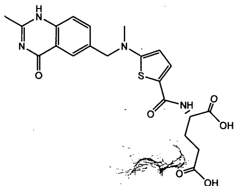
Clofarabine
