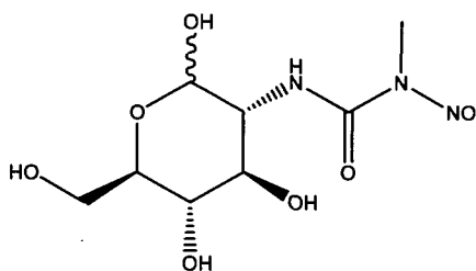
Streptozocin
