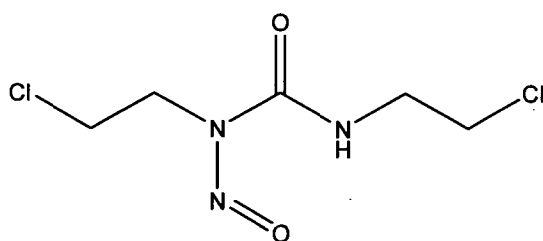
Carmustine
