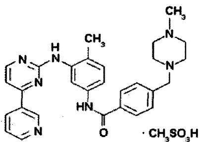
Imatinib
