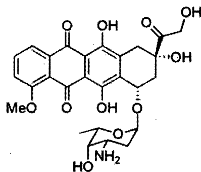
Idarubicin
