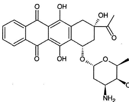
Valrubicin
