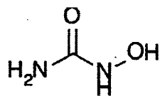
Hydroxyurea
