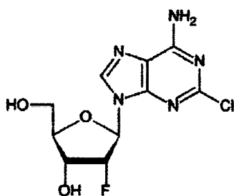
Clofarabine
