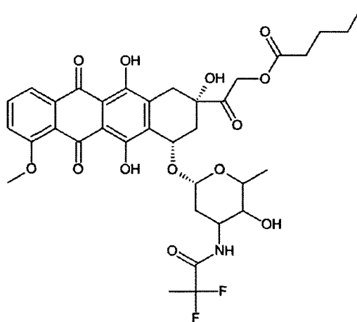
Valrubicin
