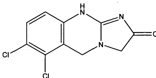
Anagrelide
