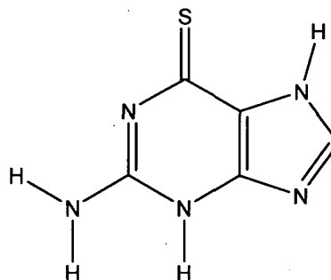
Thioguanine
