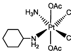
Satraplatin
