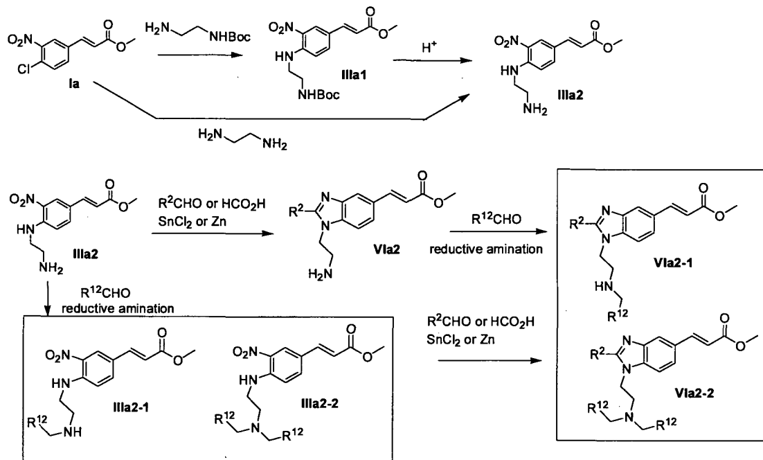
Scheme V
