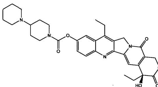
Irinotecan
