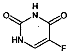
Fluorouracil
