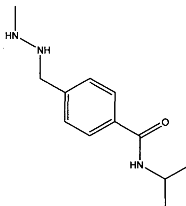
ThioTepa
