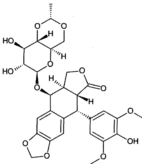
Etoposide,
