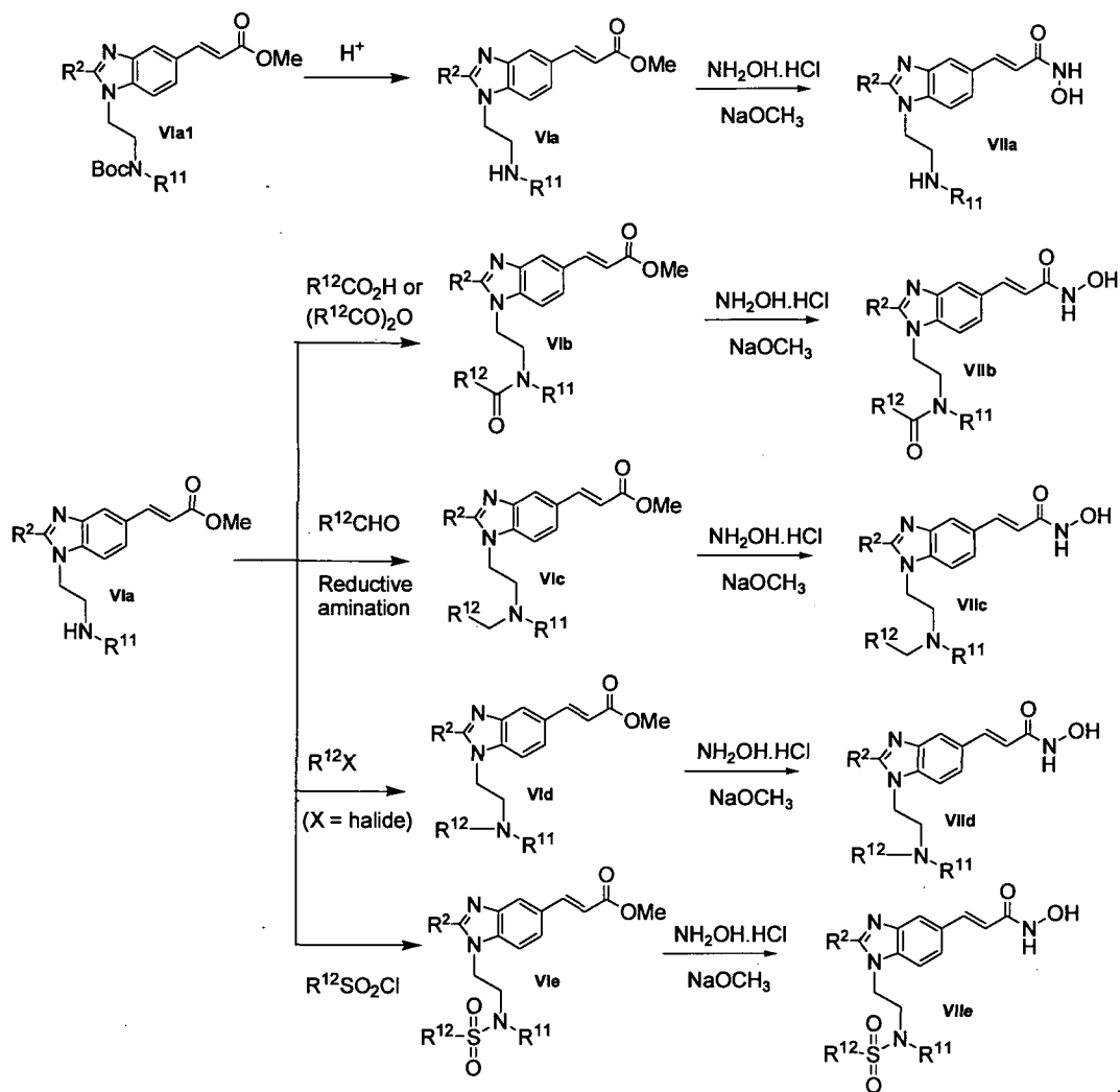
Scheme IV
