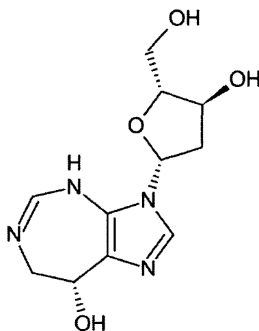
Pentostatin
