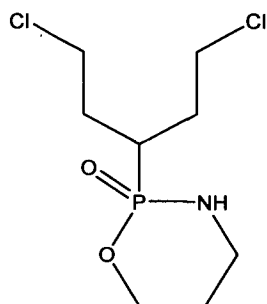
Cyclophosphamide
