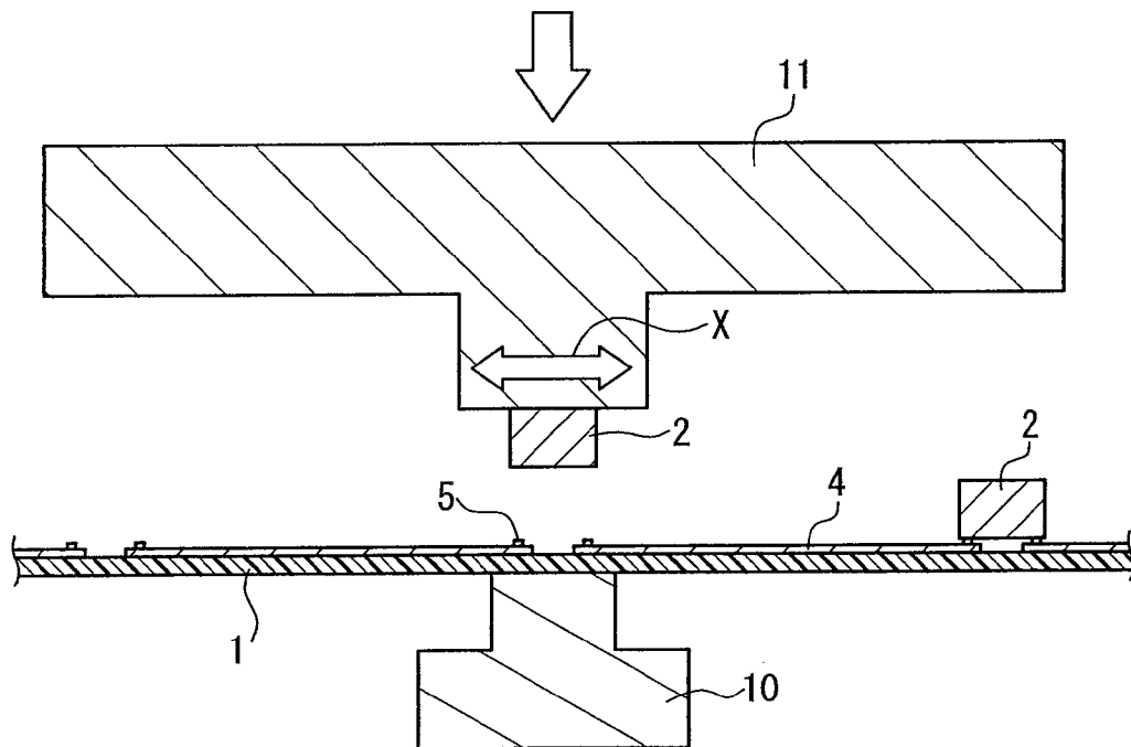
FIG. 7 PRIOR ART
