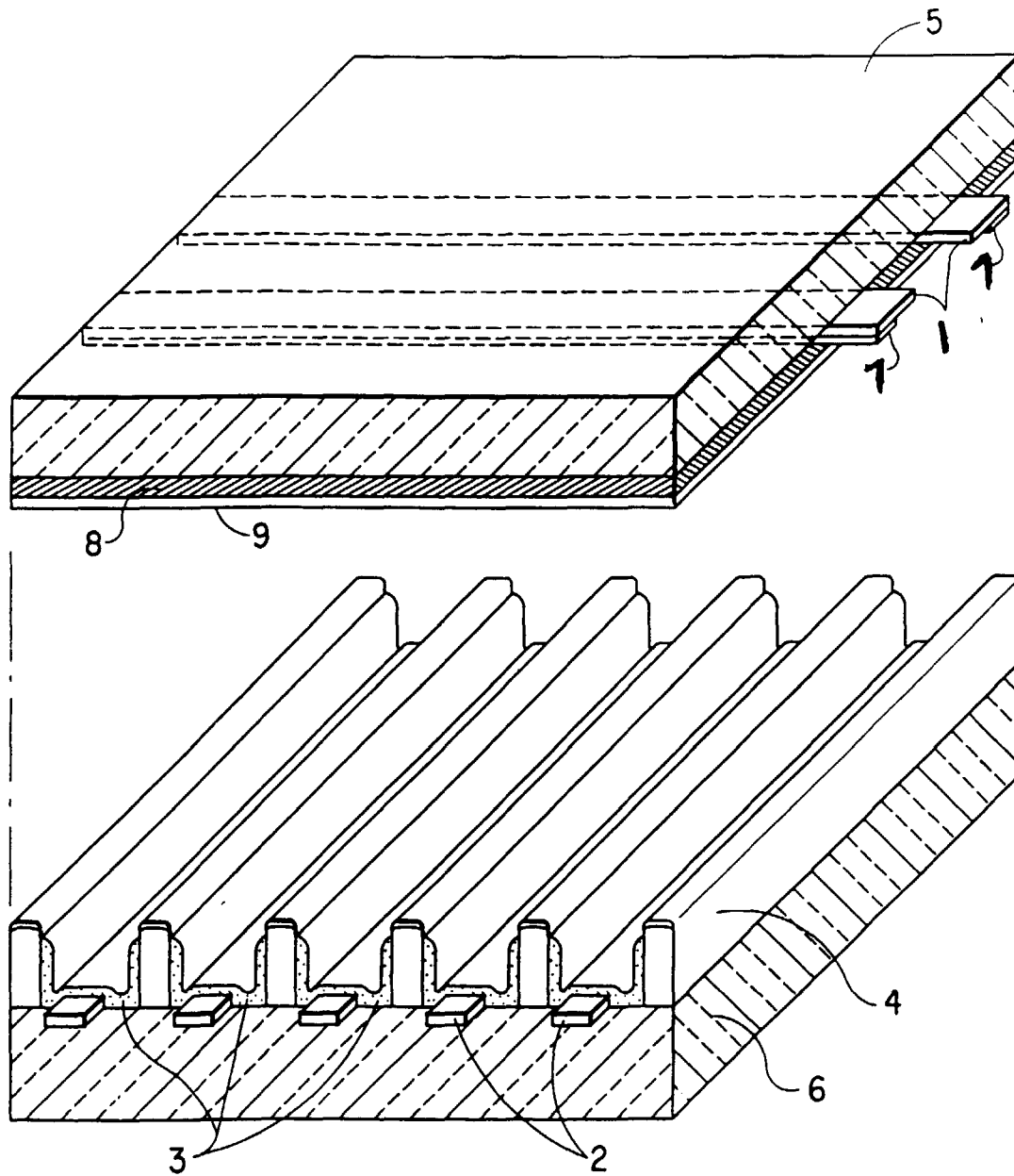
FIG. 4 (PRIOR ART)
