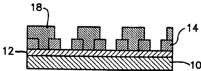
FIG. 4 PRIOR ART
