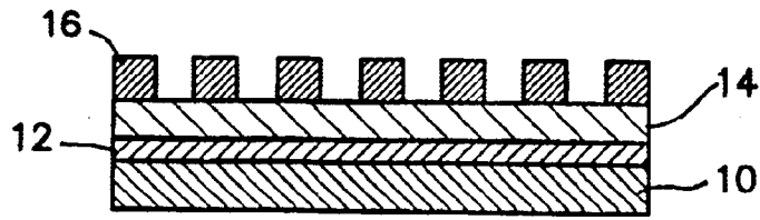
FIG. 1 PRIOR ART
