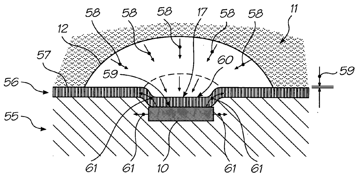
FIG. 47 (PRIOR ART)
