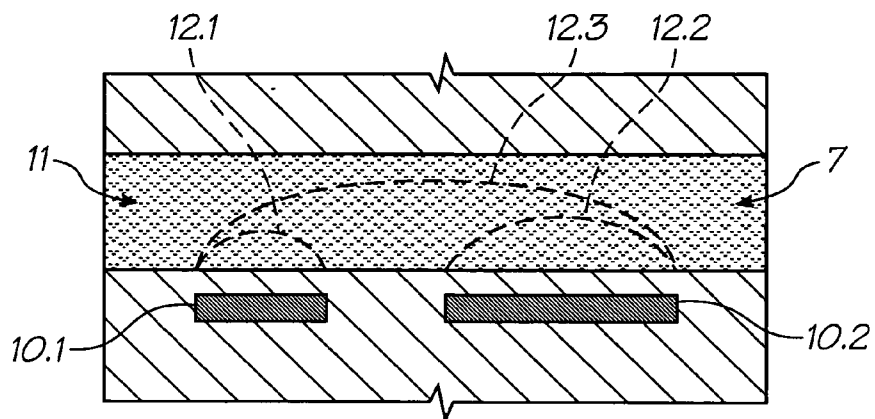
FIG. 52 (PRIOR ART)
