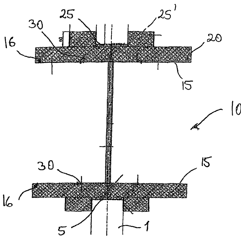
Fig. 1 PRIOR ART
