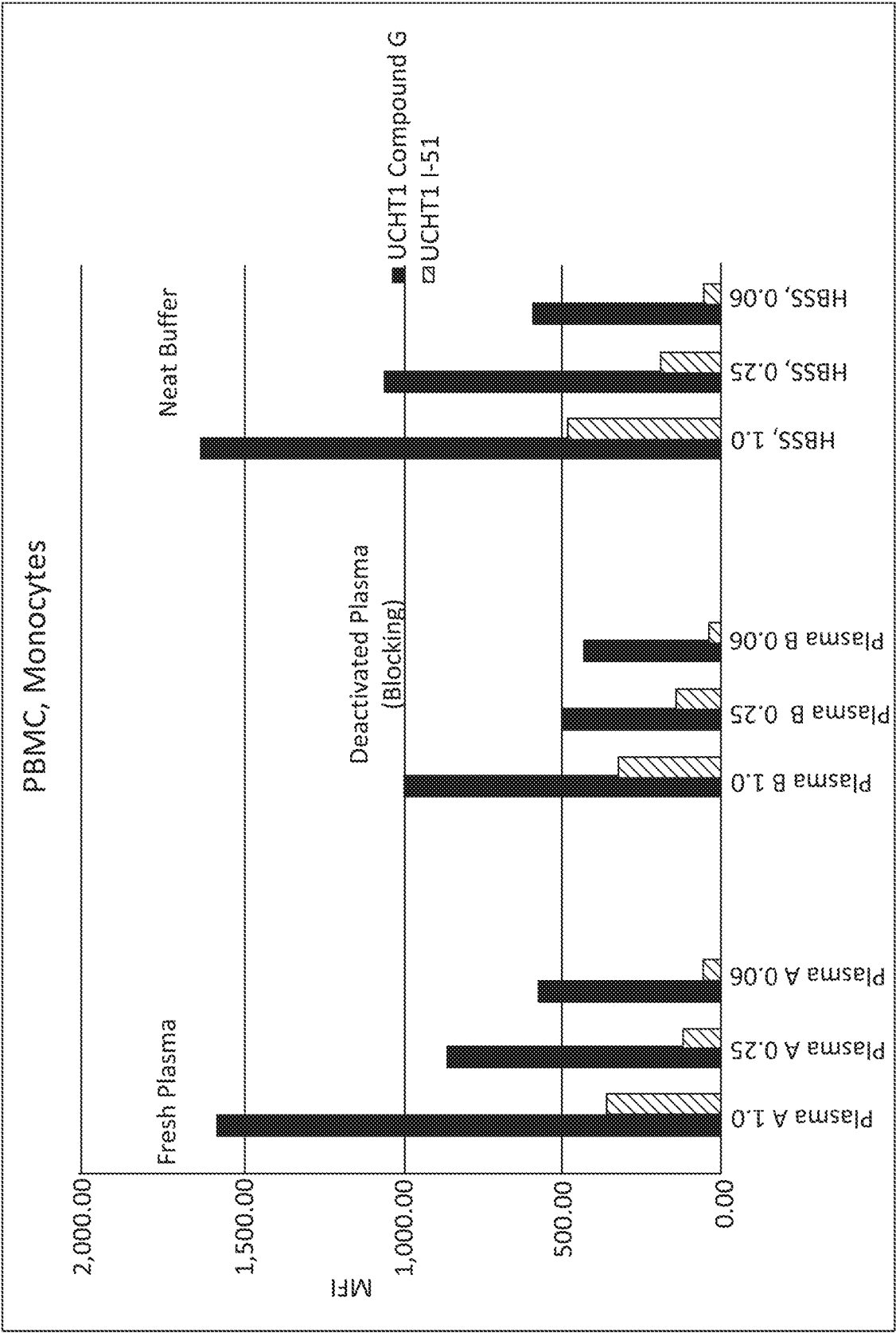
FIG. 26A 0% Glycine
