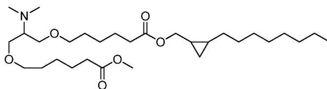
Compound 52
