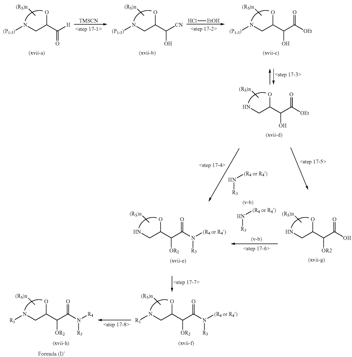
Scheme 15 Alternative synthetic route of morpholine compounds.
