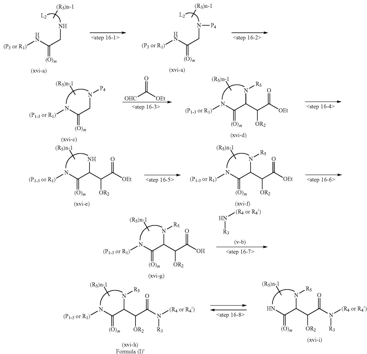
Scheme 14 Alternative synthetic route of compounds (xvi-h) identical to the compound represented Formula (I) wherein G represents nitrogen group.
