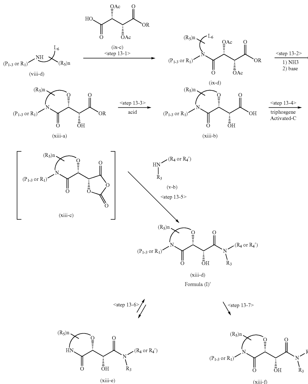
Scheme 11 Alternative synthetic route of optically active compounds (xiii-f) subset of compounds (x-e)
