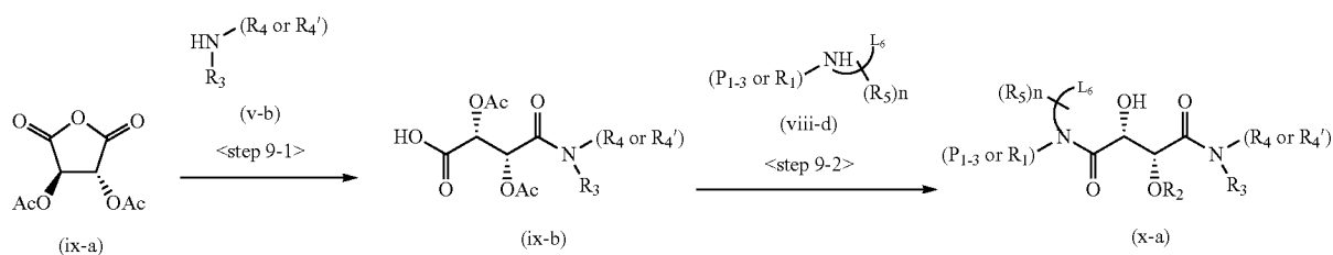
Scheme 5 Synthetic route of optically active compounds (x-b)
