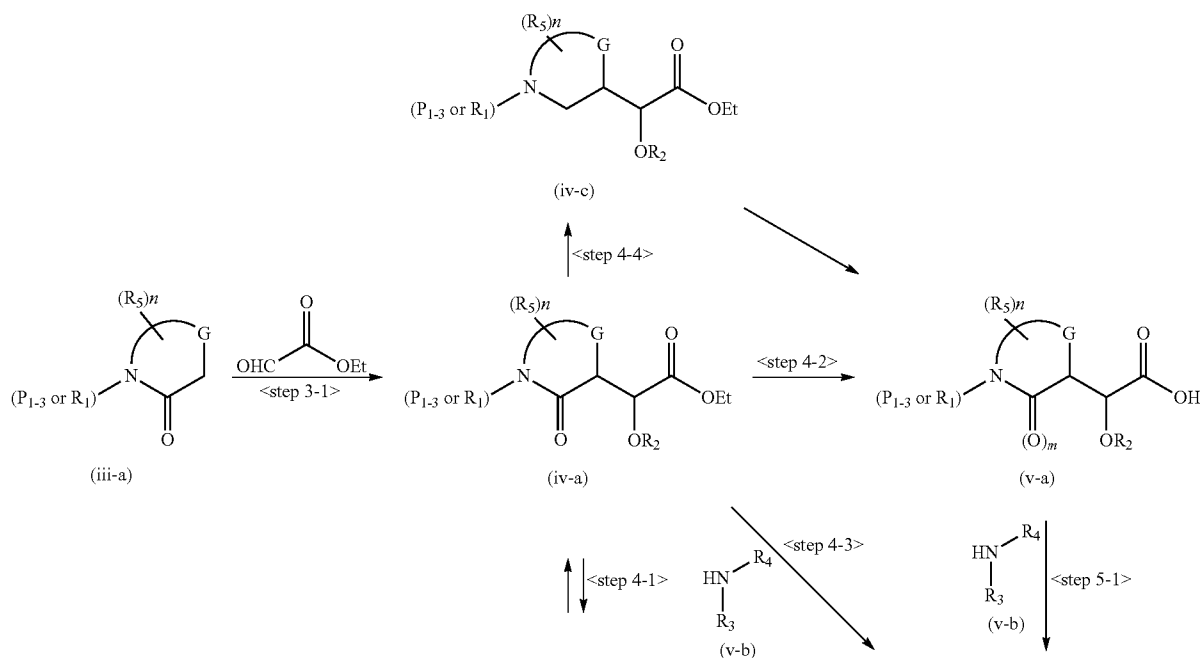
Scheme 2 Synthetic route of Example compounds and combination compounds. (Reaction scheme 2)
