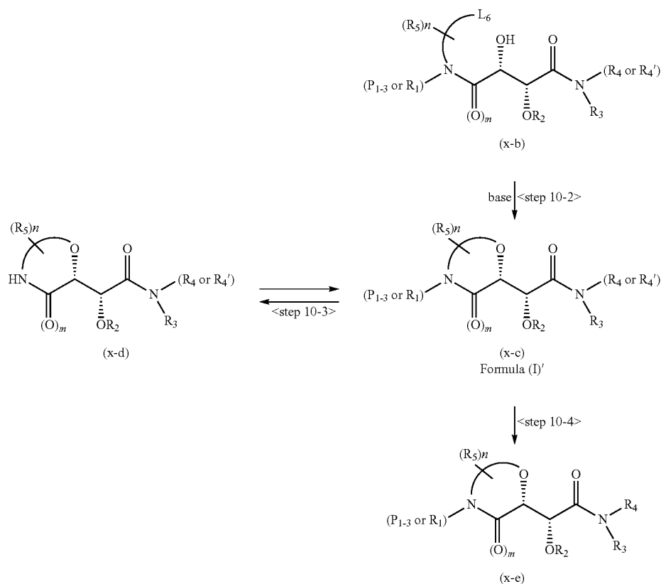
Scheme 6 Synthetic route of optically active compounds (x-c) and (x-e) (Reaction scheme 6)
