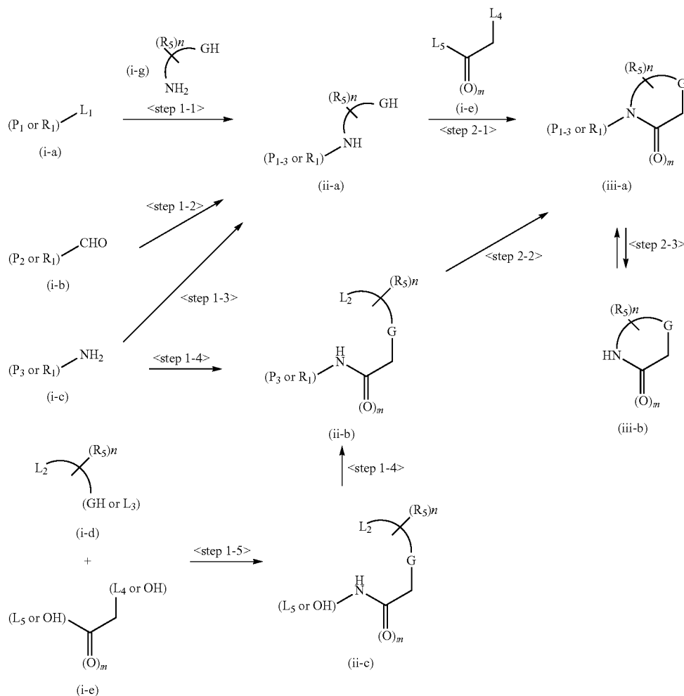
Scheme 1 Synthetic route of the key intermediate (iii-a) (Reaction scheme 1)
