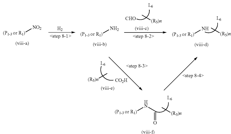
Scheme 4 Synthetic route of intermediate compounds (viii-d) (Reaction scheme 4)
