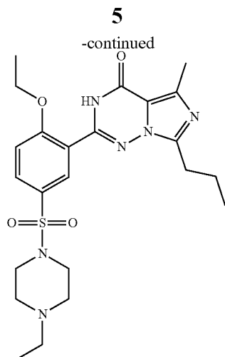
Vardenafil
