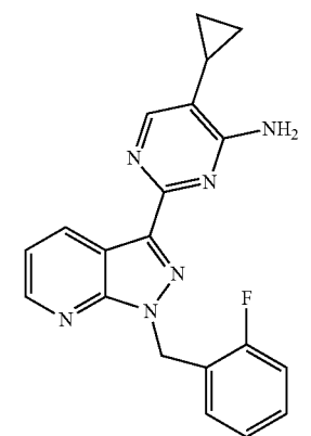
BAY 41-2272
