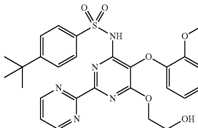
Bosentan
