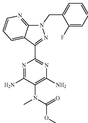
Riociguat
