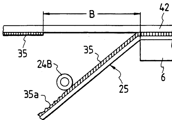
FIG. 19 PRIOR ART
