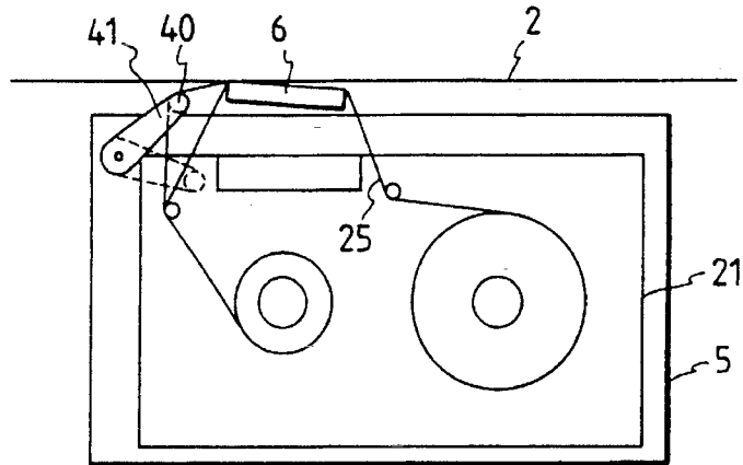
FIG. 17 PRIOR ART
