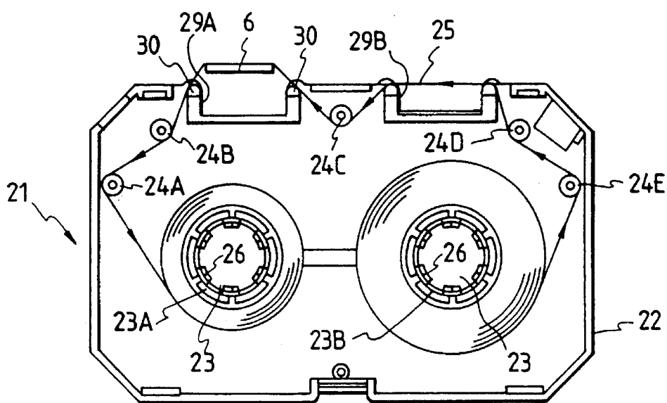
FIG. 14 PRIOR ART
