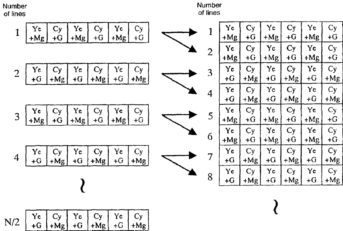
(a) Short signal before interpolation processing
