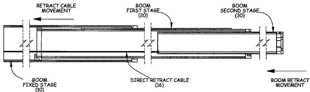
TELESCOPIC BOOM DETAIL VIEW DIRECT RETRACT CABLE
