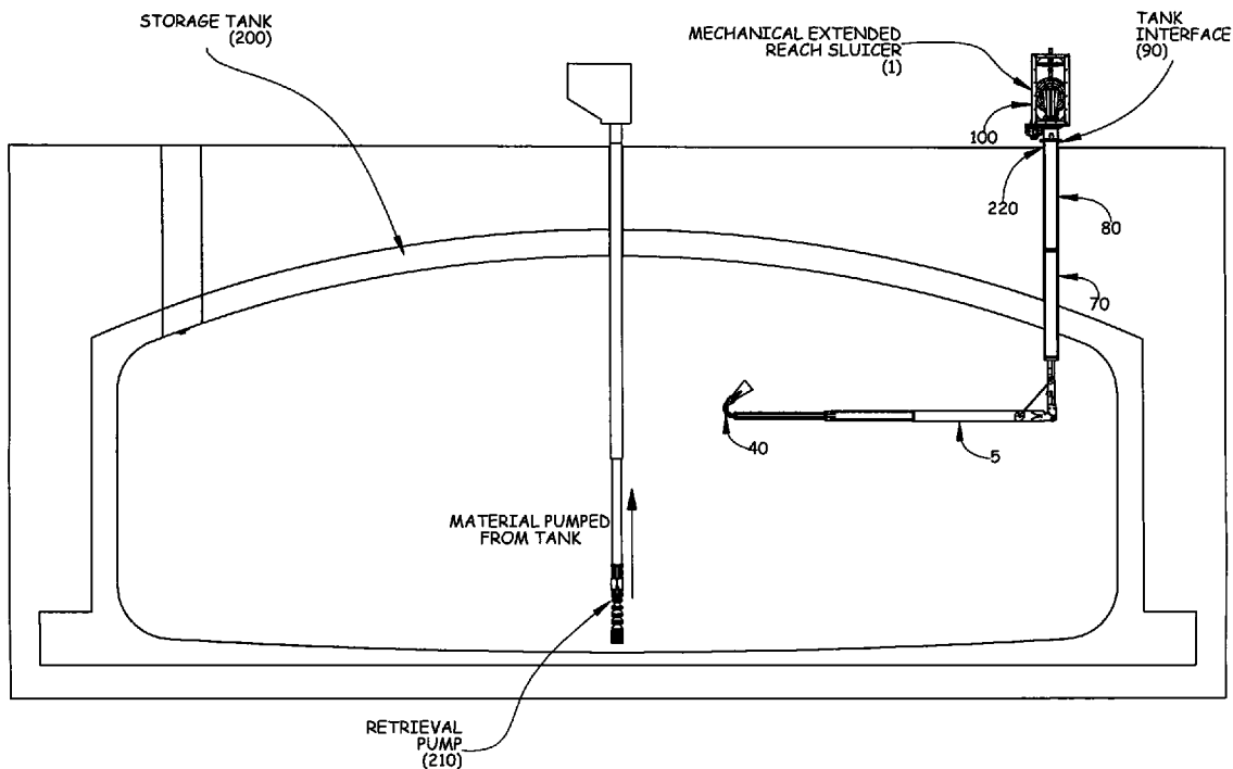
STORAGE TANK CROSS SECTION VIEW
