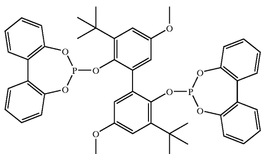
Bidentate Phosphite Ligand
