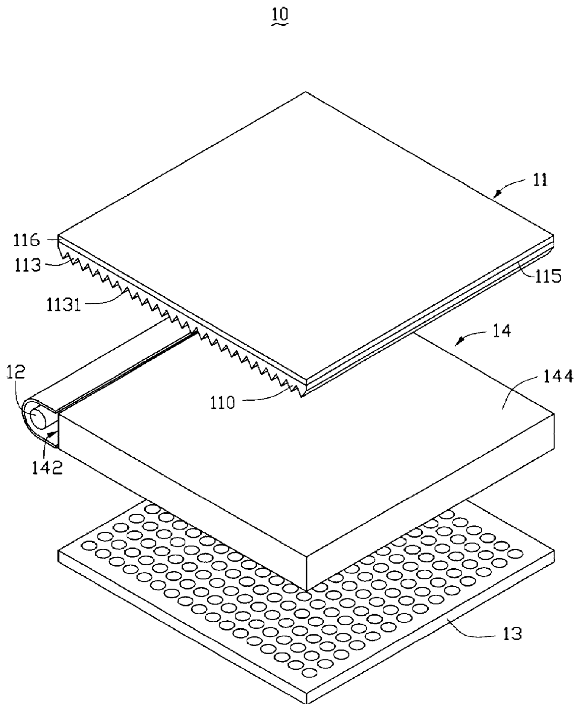
FIG. 5 (RELATED ART)
