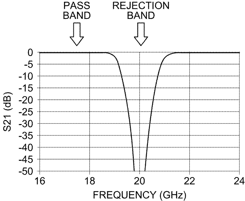
PASS CHARACTERISTICS OF BAND REJECTION FILTER
