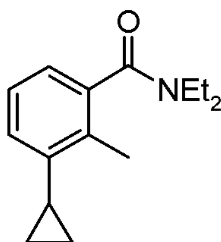
3-Cyclopropyl- N,N -diethyl-2-methyl-benzamide 7
