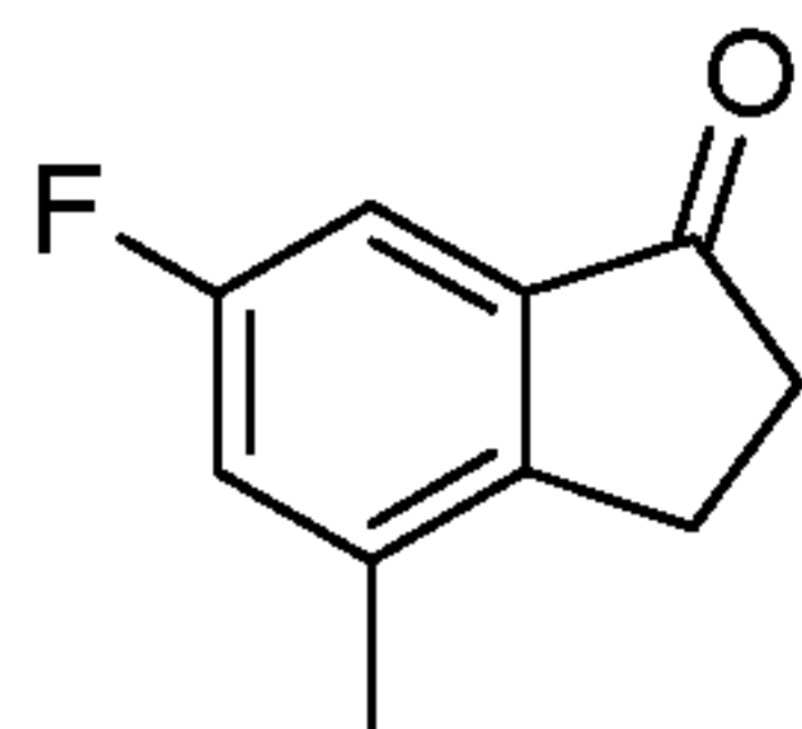
Scheme J, Step X: Indanone Synthesis 6-Fluoro-4-methyl-2,3-dihydro-1H-inden-1-one
