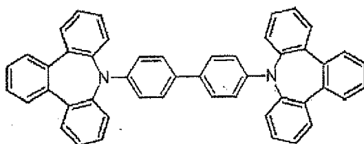
EB-3: E_a=1.9 , I_p=5.2
