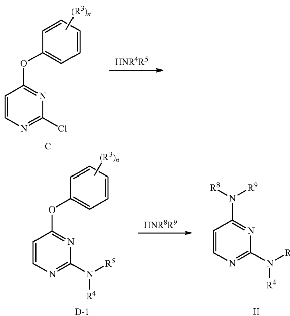
Scheme 1A:
