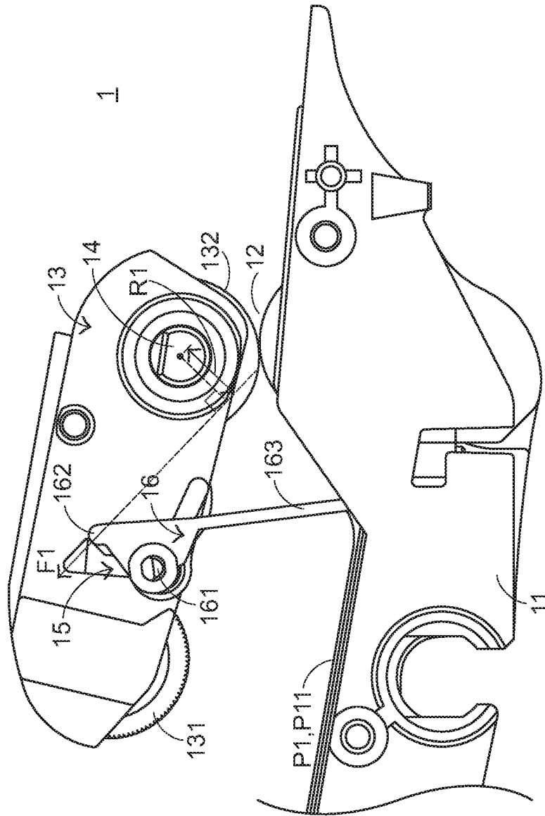
FIG.7 PRIOR ART
