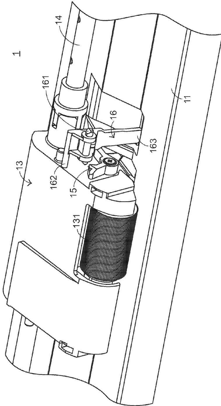
FIG.4 PRIOR ART
