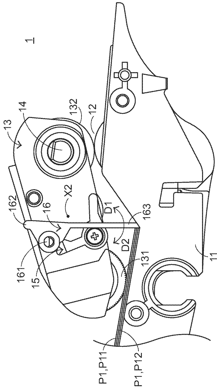
FIG.3 PRIOR ART
