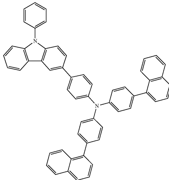
PCBNBB
