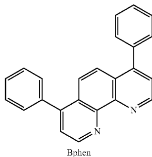
Bphen
