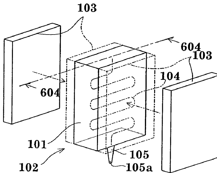
Fig.2(PRIOR ART)
