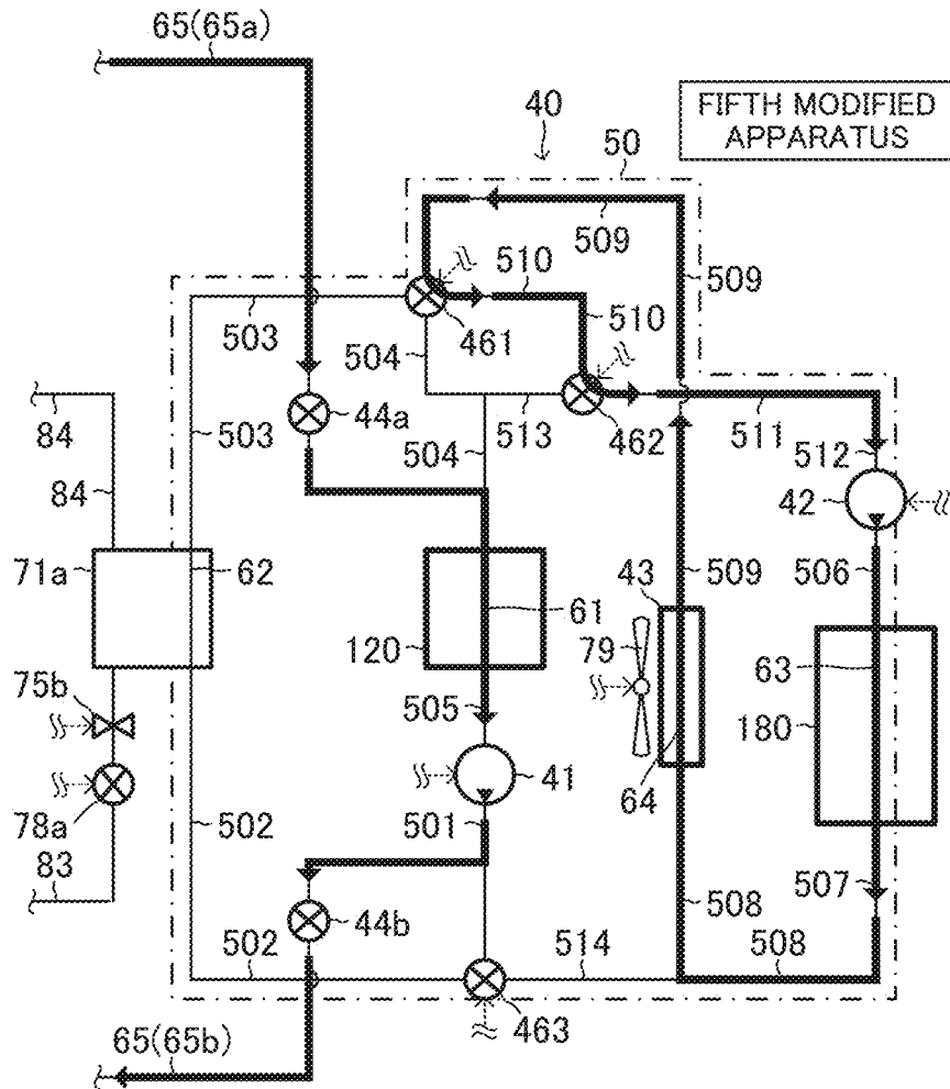
HYBRID SYSTEM CONNECTION CIRCULATION CONTROL
