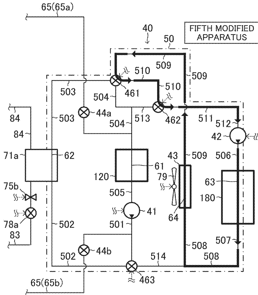
FIFTH HYBRID SYSTEM CIRCULATION CONTROL
