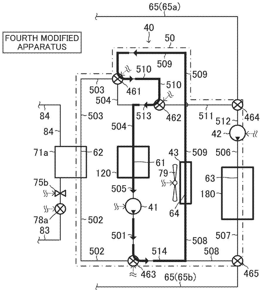
FOURTH HYBRID SYSTEM CIRCULATION CONTROL
