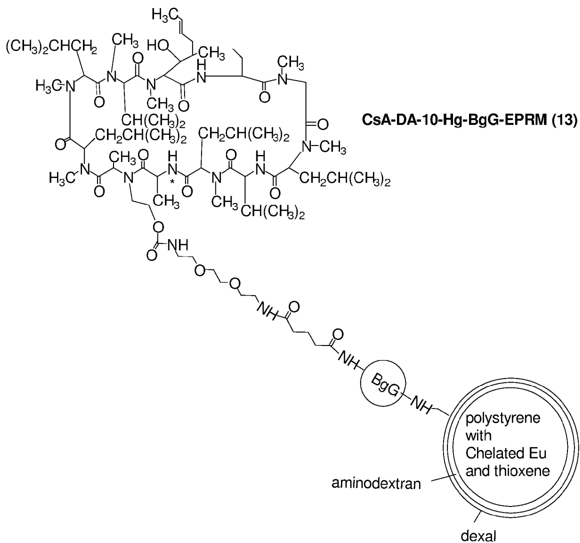
Figure 3C. CsA-DA-10-Hg-BgG-EPRM ChemiBeads
