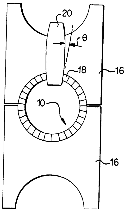
FIG. 3 PRIOR ART
