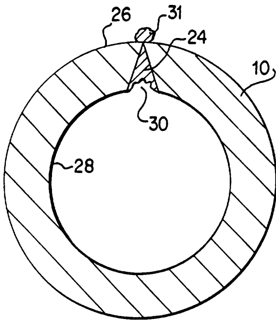
FIG. 5 PRIOR ART
