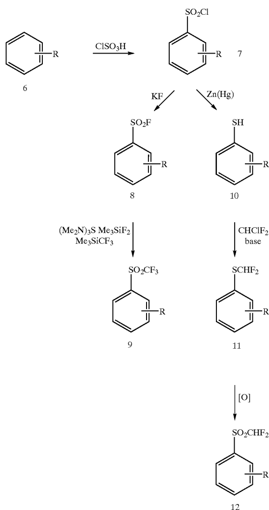
Scheme III Selected Methods of Fluorinated Aryl Sulfone Synthesis
