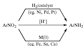
Scheme I Reduction of Nitroaryls to Aryl Amines
