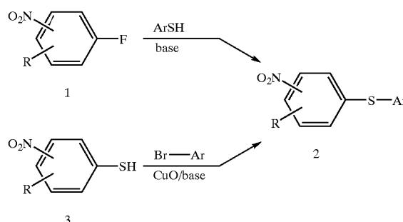
Scheme II Selected Nucleophilic Aromatic Substitution using Nitroaryls
