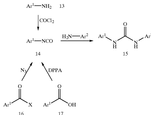
Scheme IV Selected Methods of Non-Symmetrical Urea Formation
