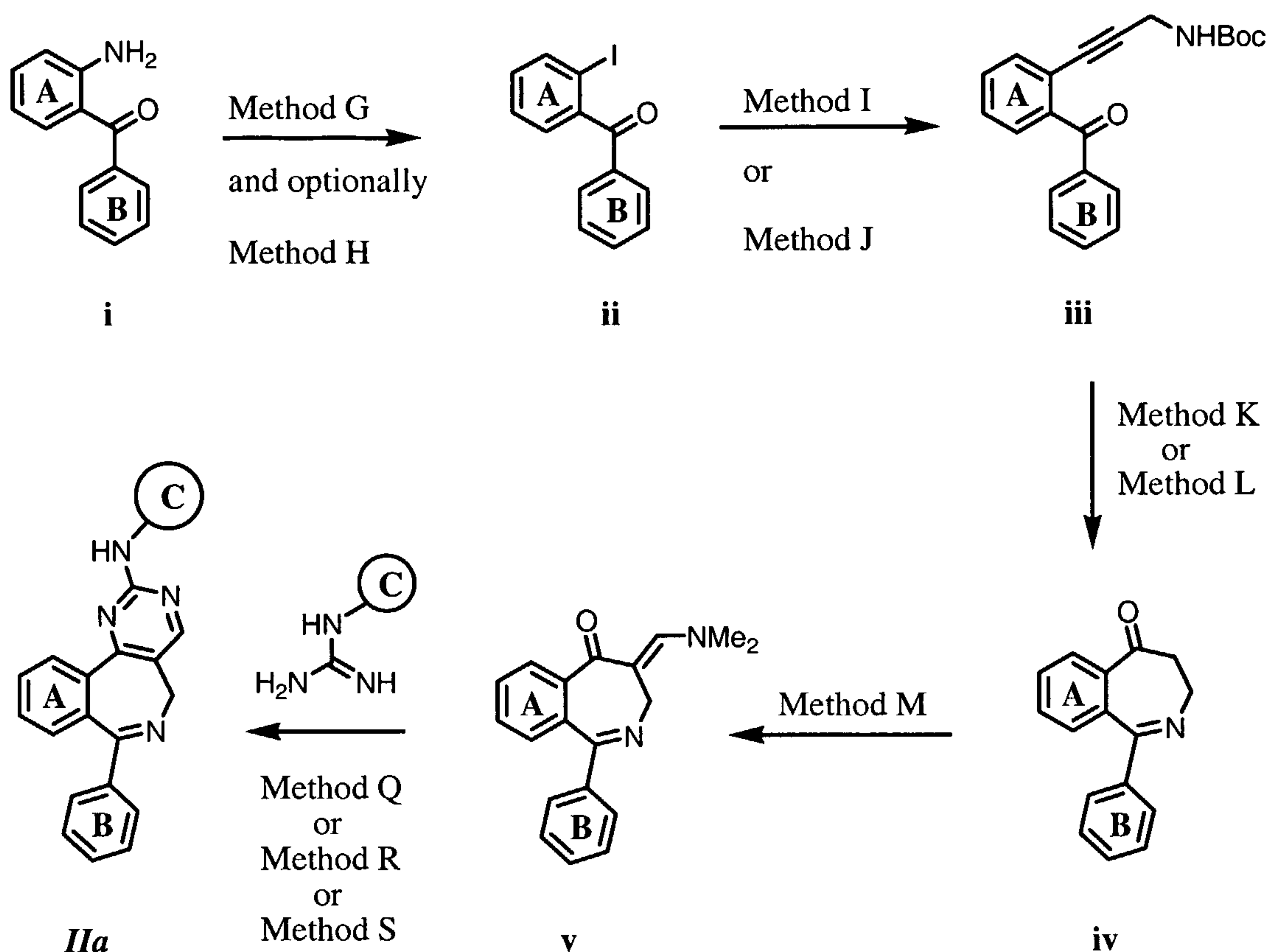
Scheme 1: General route for the synthesis of N -Aryl-(7-phenyl-5 H -benzo[ c ]pyrimido-[4,5- e ]azepin-2-yl)-amines
