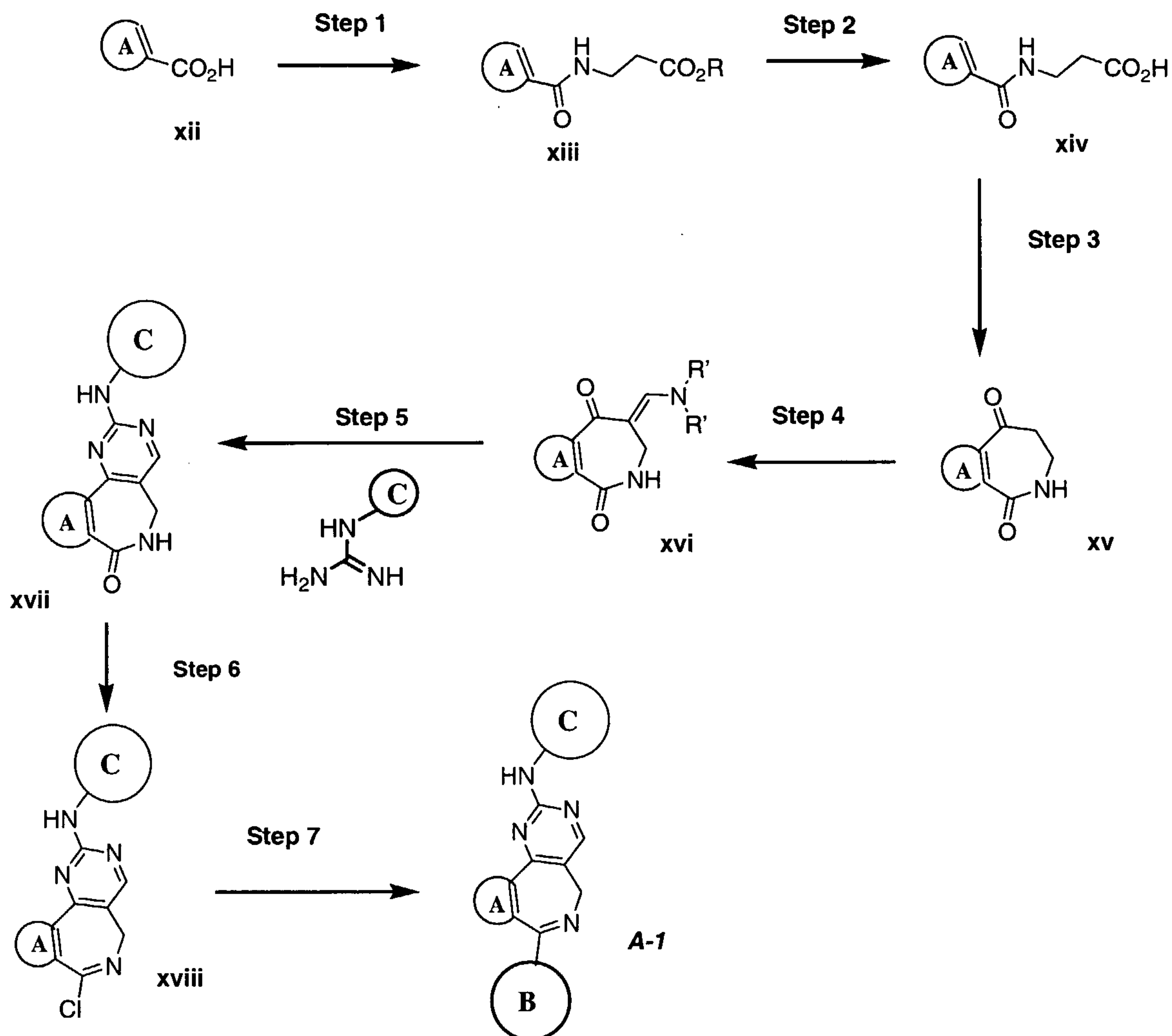
Scheme 3: Alternative route for the synthesis of compounds of formula (A-1)
