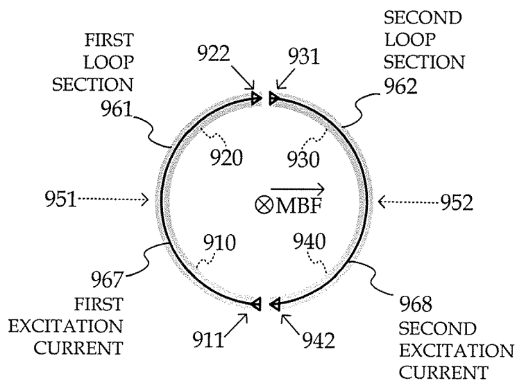
TWO LOOP SECTIONS OF DISCONTINUOUS-LOOP ANTENNA AND EXCITATION CURRENTS
