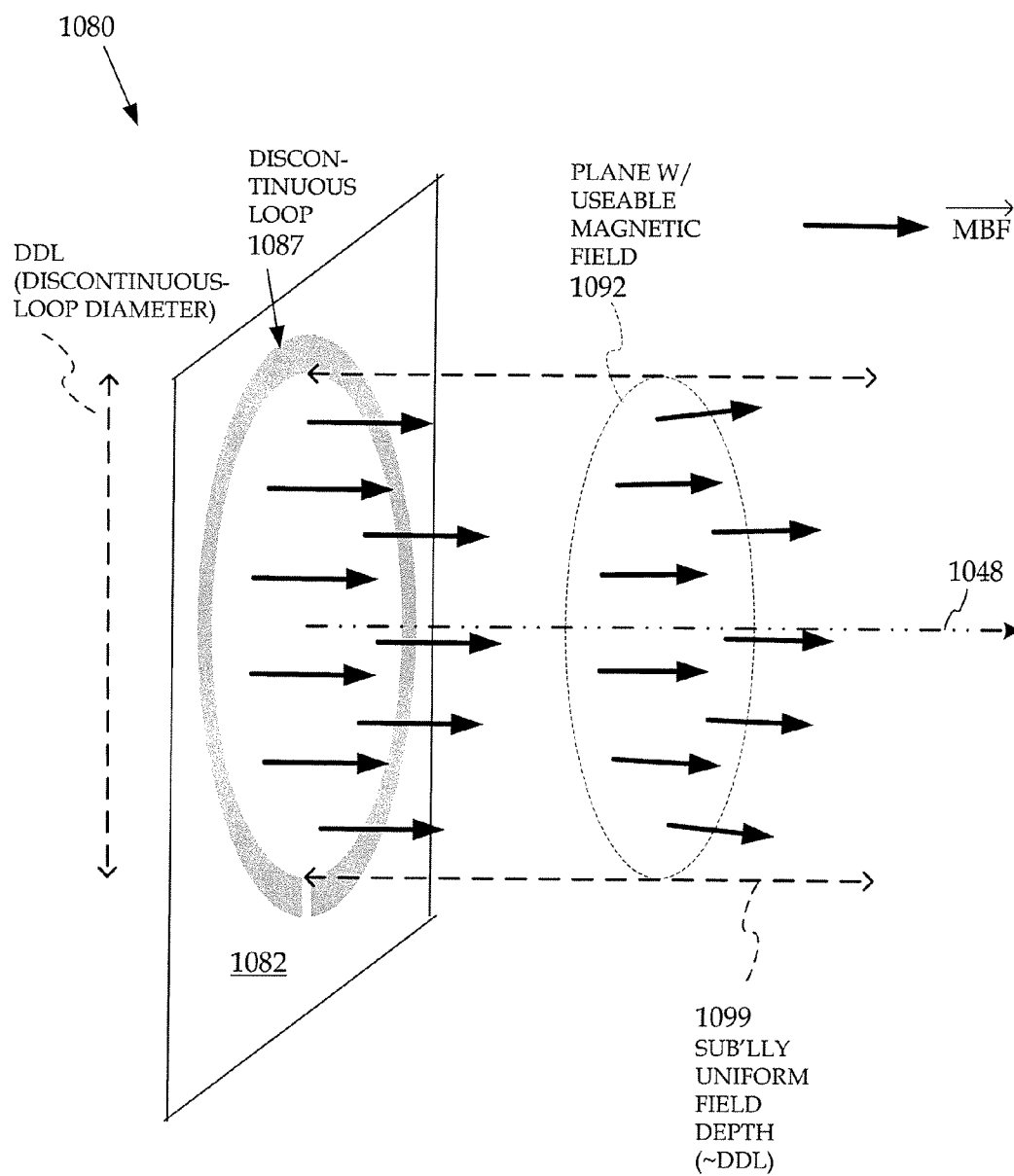
RFID READER DISCONTINUOUS-LOOP ANTENNA WITH UNIFORM MAGNETIC FIELD IN THE NEAR-FIELD
