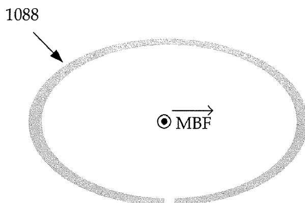
SINGLE LOOP SECTION OF DISCONTINUOUS-LOOP ANTENNA SHAPED ELLIPTICALLY
