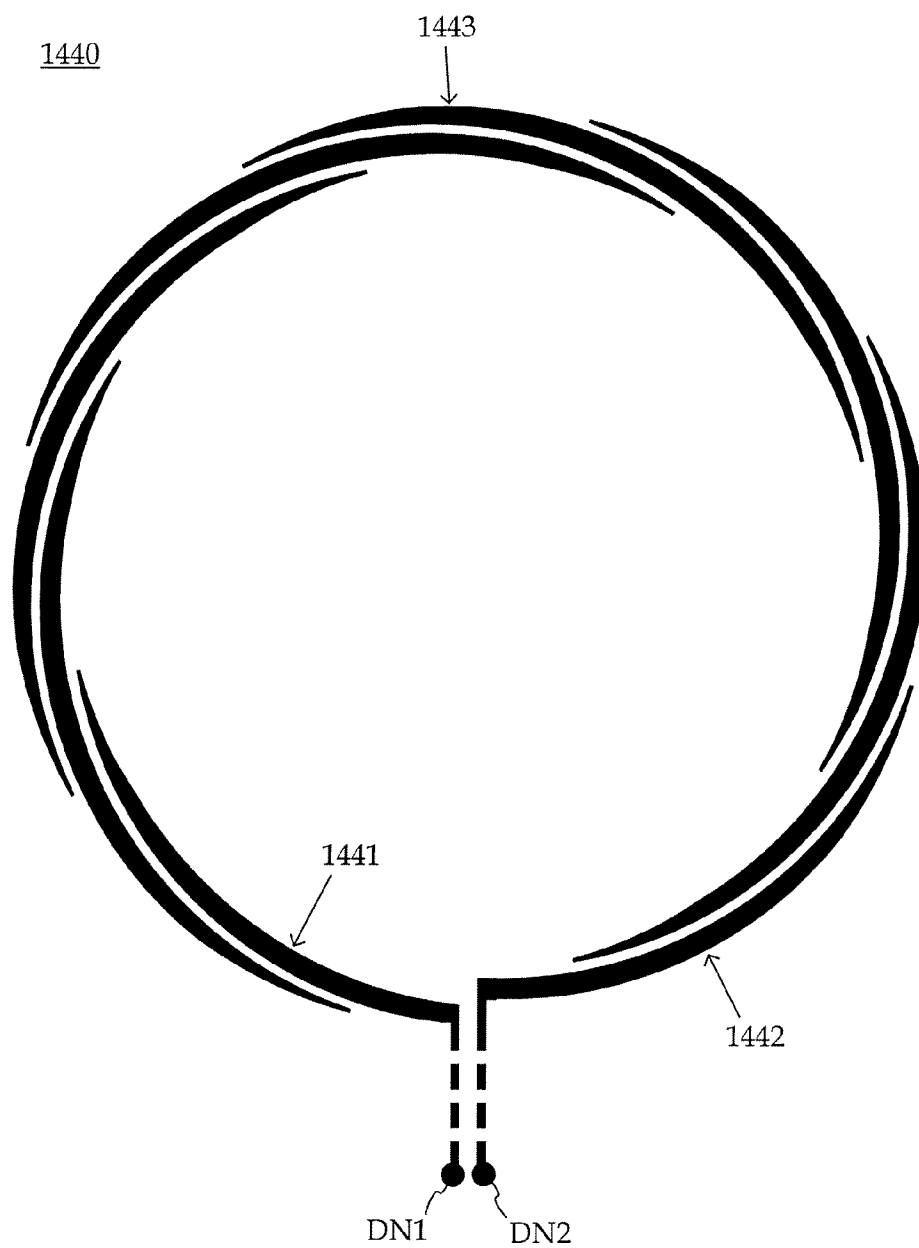
DISCONTINUOUS-LOOP ANTENNA WITH CONDUCTORS HAVING SLANTED ENDS
