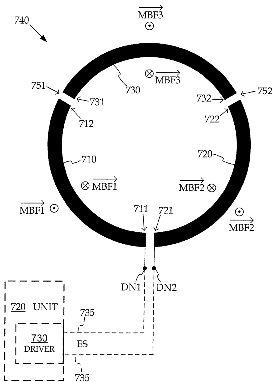
DISCONTINUOUS-LOOP ANTENNA WITH SINGLE LOOP SECTION, HAVING THREE CONDUCTORS IN SINGLE ROW
