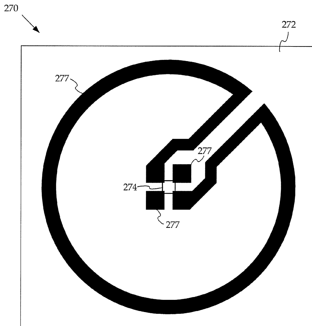
RFID TAG WITH "LOOP" ANTENNA
