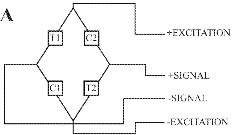
Full Bridge Schematic 1
