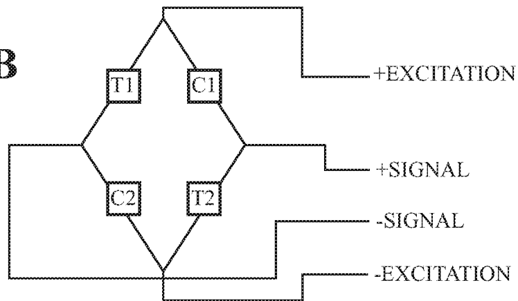
Full Bridge Schematic 2
