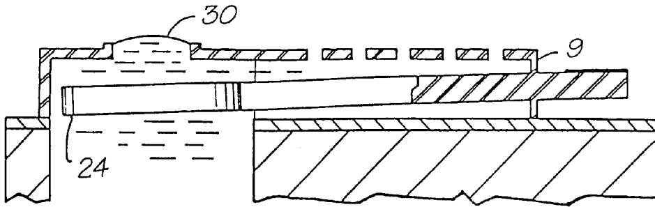
FIG. 3 (PRIOR ART)
