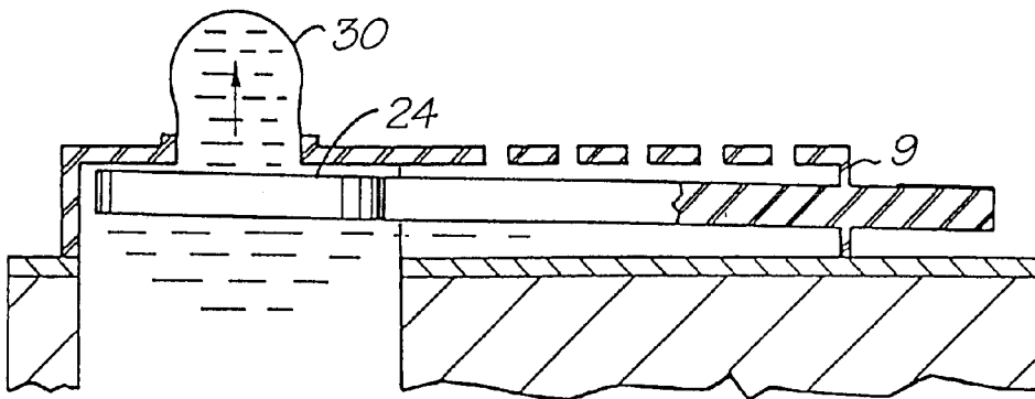
FIG. 4 (PRIOR ART)
