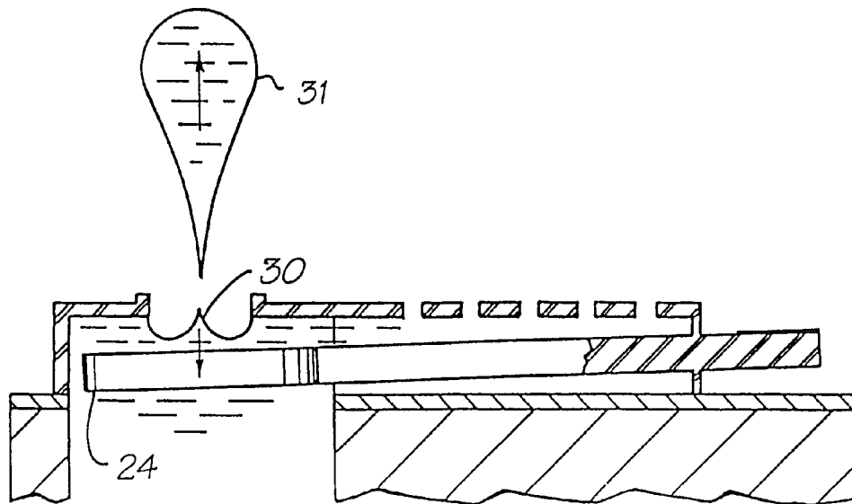
FIG. 5 (PRIOR ART)
