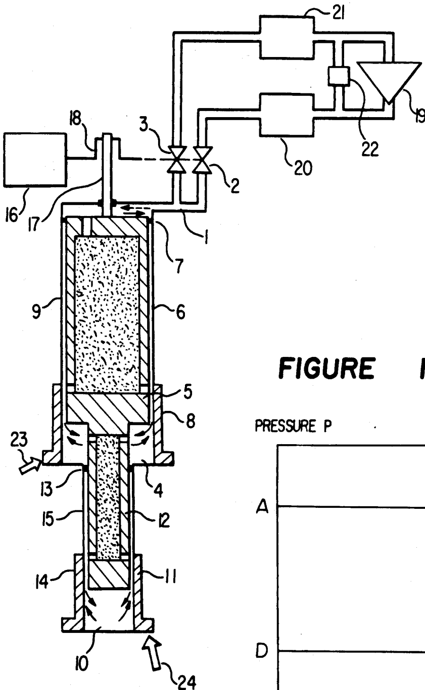
FIGURE 10 PRIOR ART
