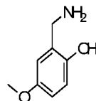
5-Methoxysalicylamine (5-MoSA)
