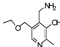
Ethylpyridoxamine (EtPM)
